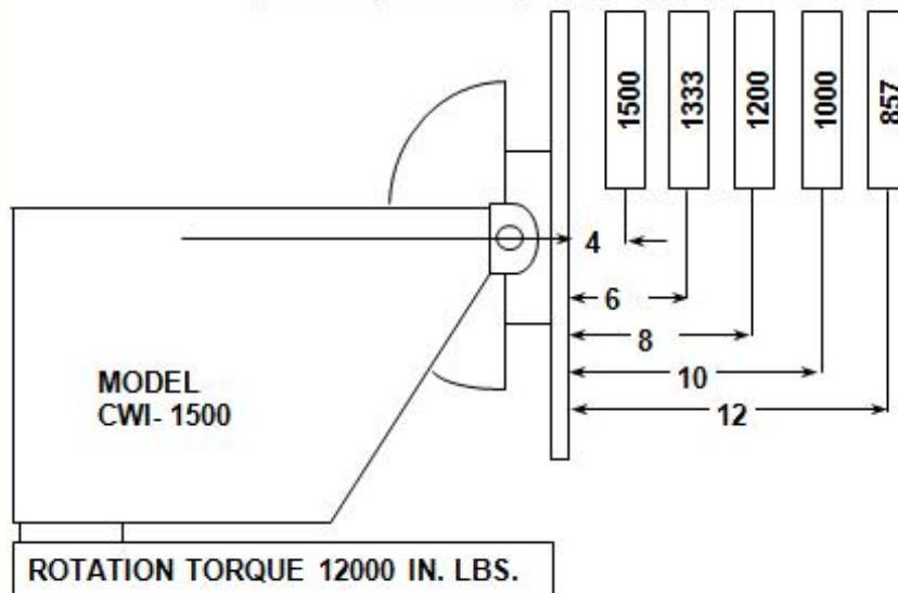
Overhung Load Capacity Chart
