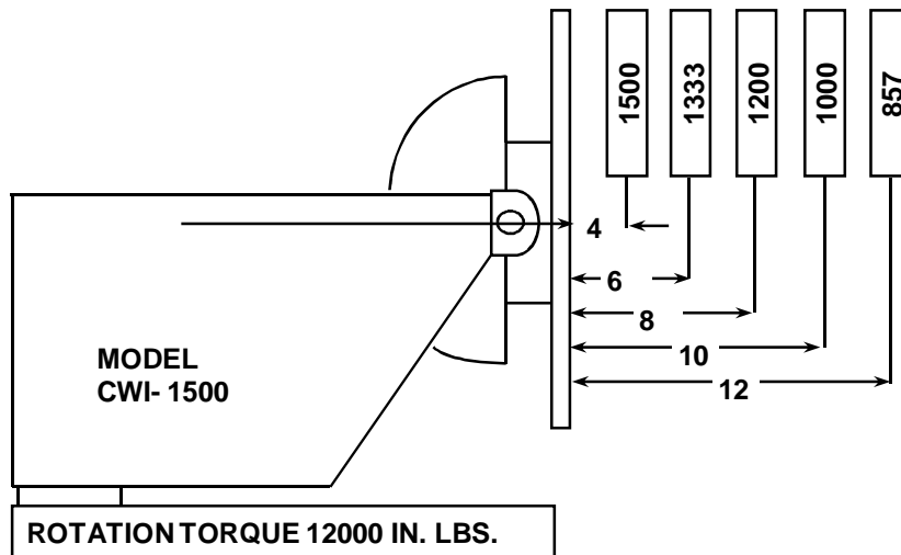
Overhung Load Capacity Chart
